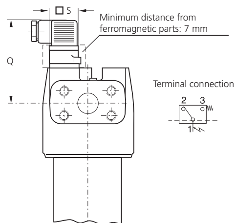
Version with integrated electrical clogging indicator SAE-flange (6000 psi)
